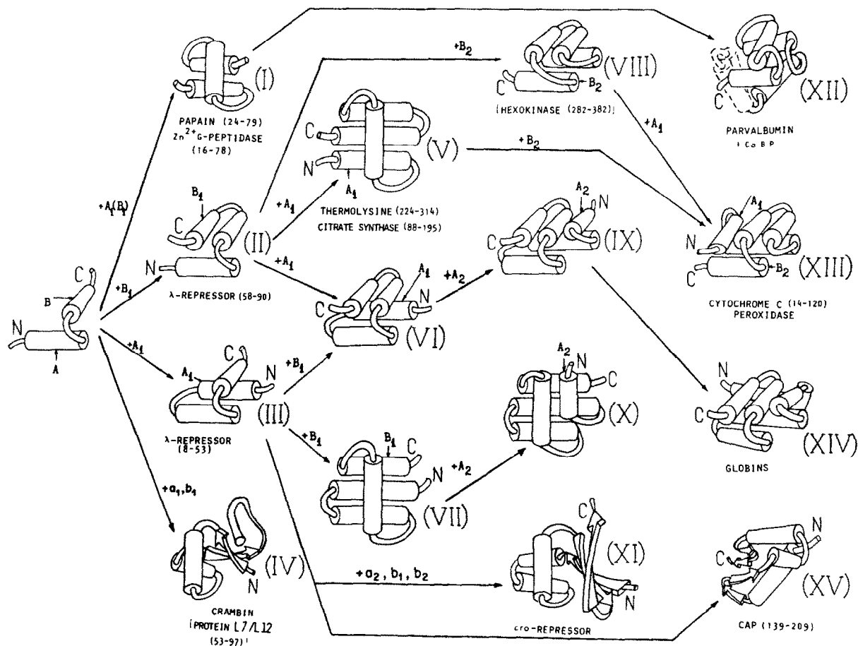
Fig.4. A scheme of growing the structures using a stepwise addition of \alpha -helices when an \alpha\alpha -corner is taken as the initiating complex. \alpha -Helices are shown by cylinders; connections are simplified. Proteins or their regions which have corresponding structures are denoted under them. See also the text.
